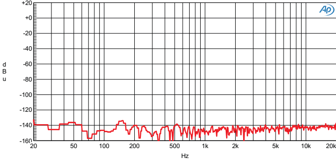
Stereo Direct Box Isolate Noise Spectrum
