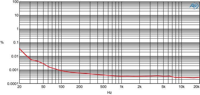
Stereo Direct Box Isolate Total Hamonic Distortion vs Frequency
