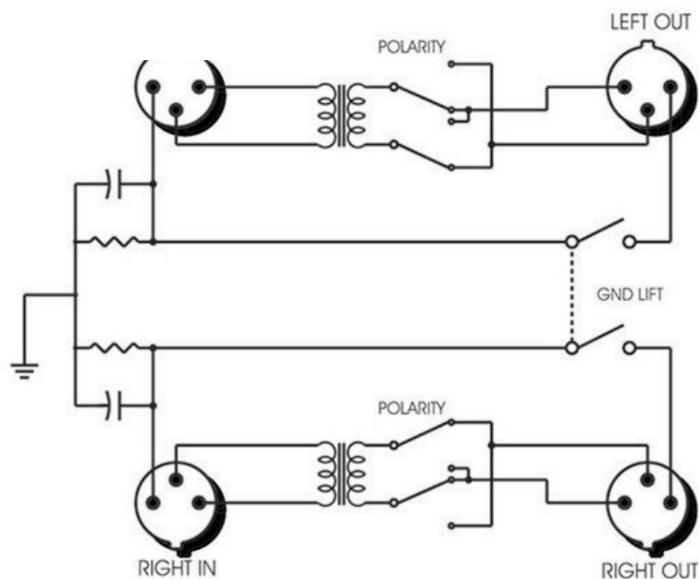
Twin-Iso Block Diagram
