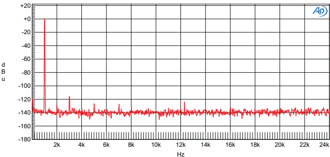
Stereo Direct Box Isolate Fast Fourier Transform
